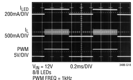
Figure 8b. PWM Dimming Waveforms
