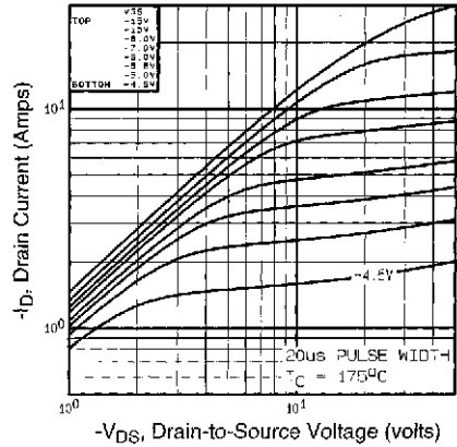
Fig 2. Typical Output Characteristics, T_C=175^\circ C
