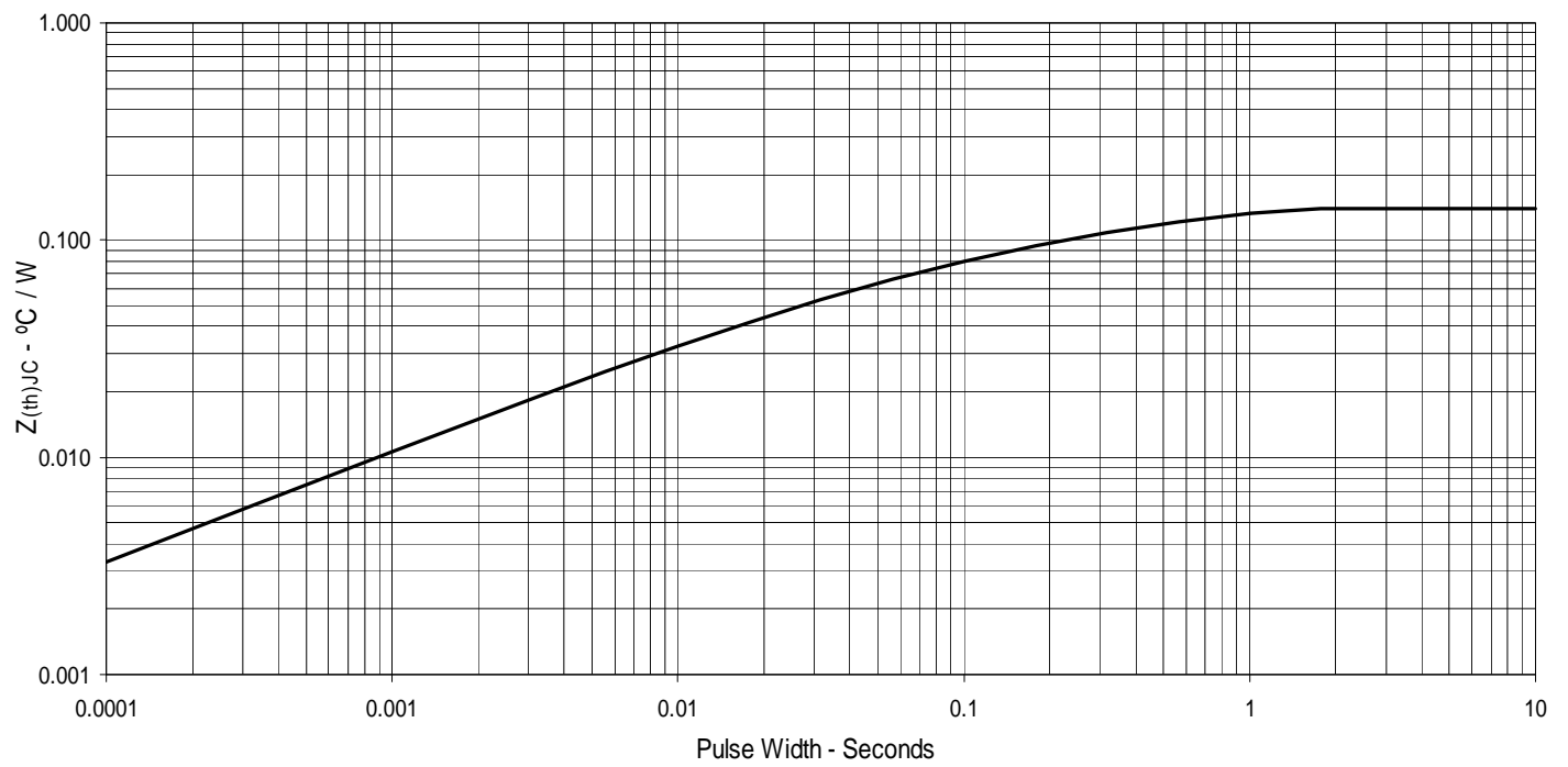
Fig. 12. Maximum Transient Thermal Impedance
