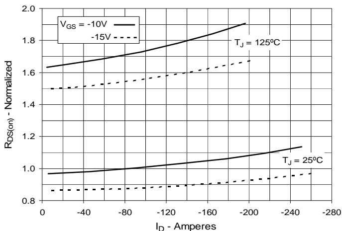
Fig. 5. R_{DS(on)} Normalized to I_D = -85\text{A} vs. Drain Current
