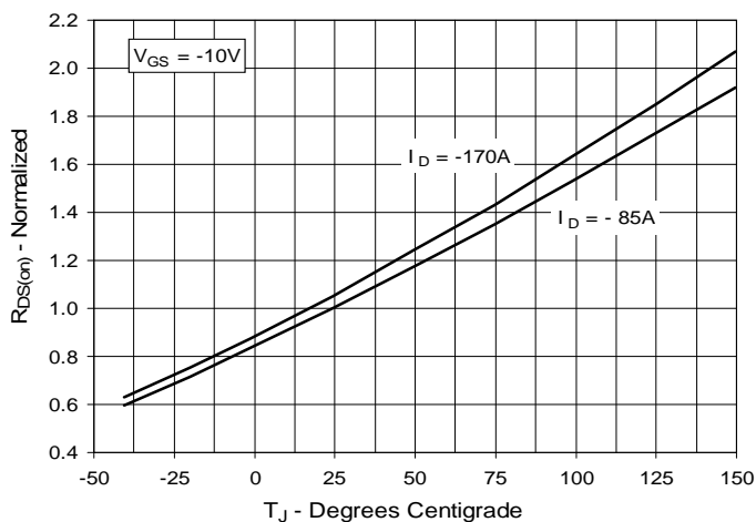
Fig. 4. R_{DS(on)} Normalized to I_D = -85\text{A} vs. Junction Temperature
