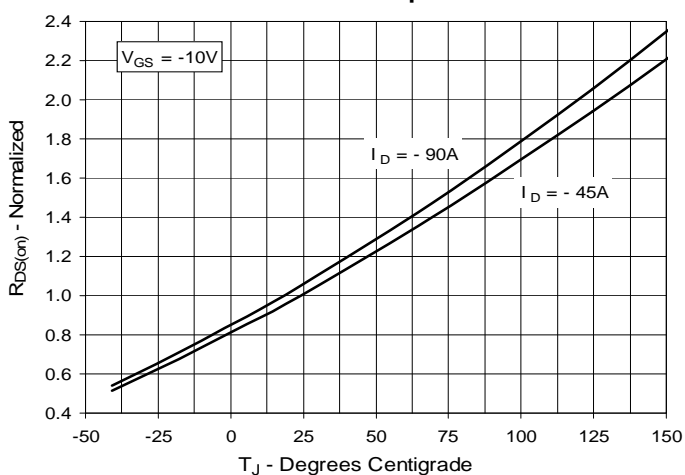
Fig. 4. R_{DS(on)} Normalized to I_D = -45A . Junction Temperature
