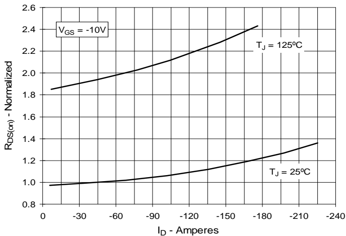
Fig. 5. R_{DS(on)} Normalized to I_D = -45A . Drain Current
