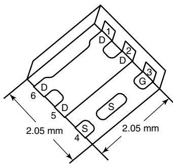
PowerPAK SC-70-6L-Single
