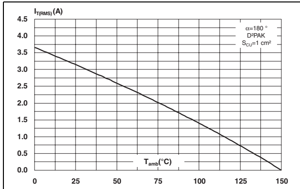
Figure 3. RMS on-state current versus ambient temperature (Epoxy printed circuit board FR4, copper thickness = 35 \mu m)
