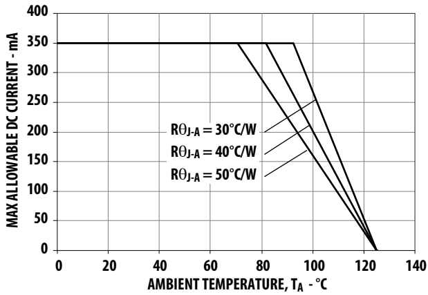
Figure 7. Maximum Forward Current vs. Ambient Temperature. Derated based on T_{JMAX} = 125^\circ\text{C} , R_{\theta J-A} = 30^\circ\text{C/W} , 40^\circ\text{C/W} and 50^\circ\text{C/W} .
