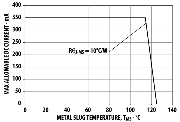
Figure 8. Maximum Forward Current vs. Metal Slug Temperature. Derated based on T_{JMAX} = 125^\circ\text{C} , R_{\theta J-MS} = 10^\circ\text{C/W} .
