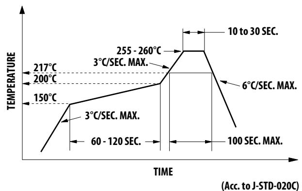
Figure 20. Recommended Reflow Soldering. (Acc. to J-STD-020C)
