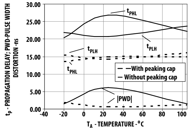
(ii) V_{DD}=3.3V , C_{peak}=100pF , R_{limit}=80\Omega
