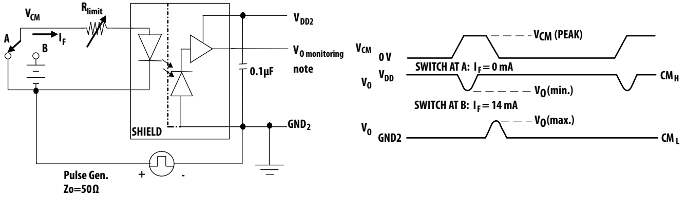
Figure 13. Test circuit for common mode transient immunity and typical waveforms.
