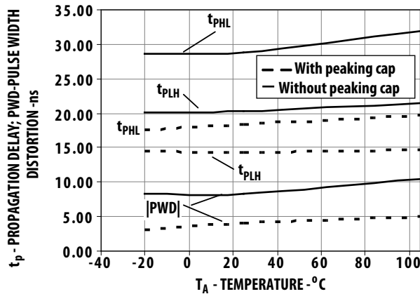
(i) V_{DD}=5V , C_{peak}=100pF , R_{limit}=220\Omega
