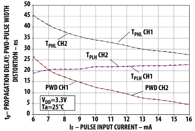
Figure 6. Typical switching speed vs. pulse input current at 3.3V supply
