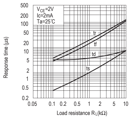
Figure 10. Response Time vs. Load Resistance
