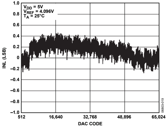
Figure 8. AD5064/AD5064-1 INL
