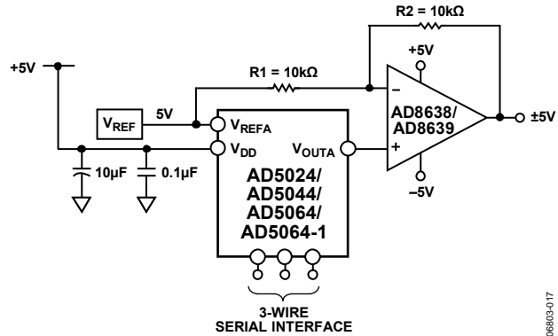
Figure 57. Bipolar Operation
