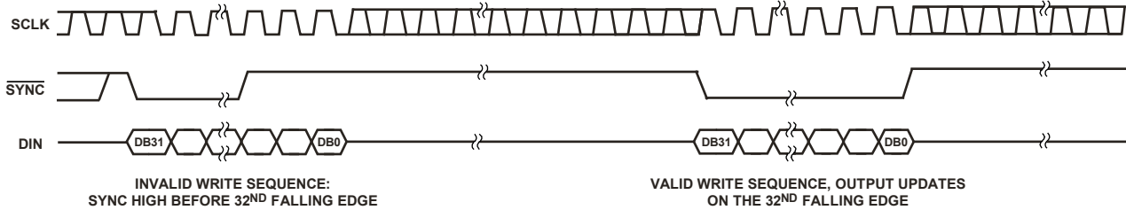
Figure 50. \overline{SYNC} Interrupt Facility
