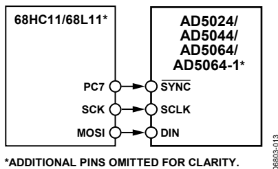
Figure 53. AD5024/AD5044/AD5064/AD5064-1 to 68HC11/68L11 Interface
