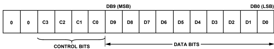
Figure 2. AD5291/AD5292 Shift Register Content
