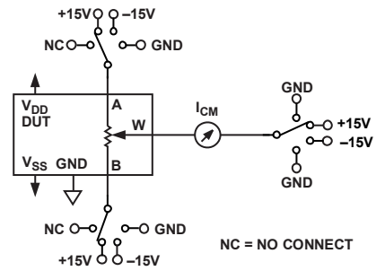
Figure 42. Common-Mode Leakage Current
