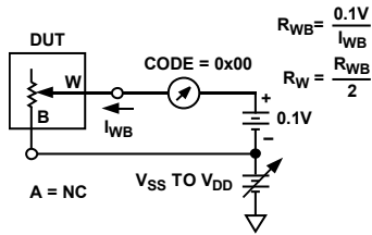
Figure 39. Wiper Resistance
