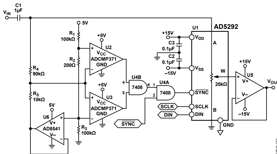
Figure 53. Audio Volume Control with Zipper Noise Reduction
