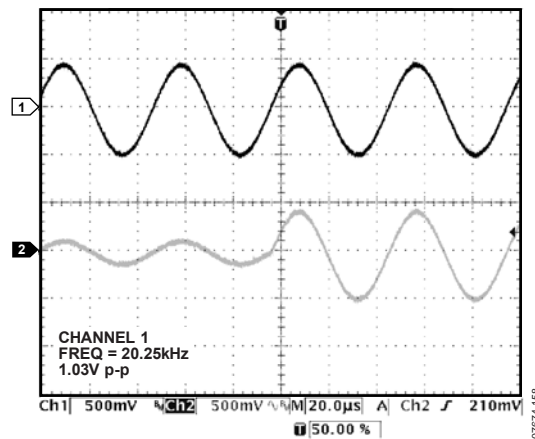
Figure 54. Zipper Noise Detector
