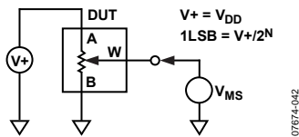
Figure 38. Potentiometer Divider Nonlinearity Error (INL, DNL)
