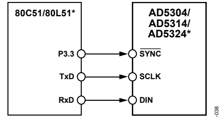
Figure 38. AD5304/AD5314/AD5324 to 80C51/80L51 Interface
