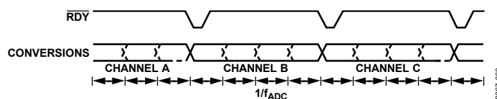
Figure 23. Channel Sequencer
