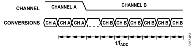
Figure 54. Fast Settling, Sinc 4 Filter
