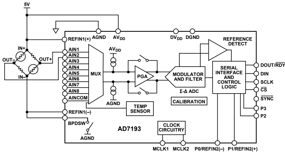
Figure 21. Basic Connection Diagram
