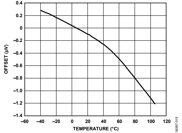
Figure 15. Offset vs. Temperature (Gain = 128, Chop Disabled)
