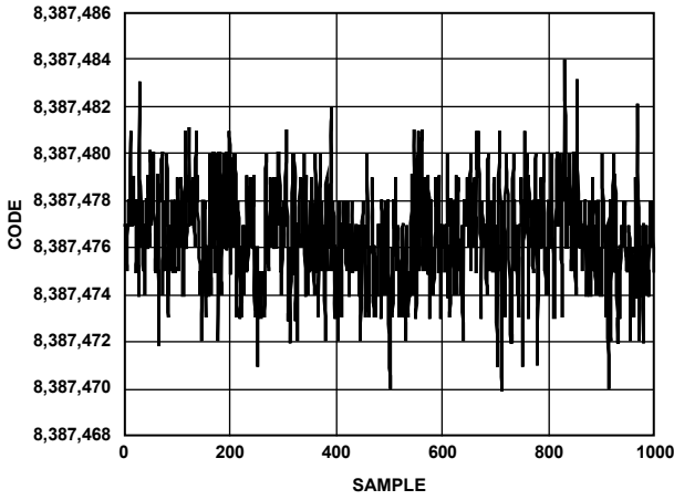
Figure 6. Noise ( V_{REF} = AV_{DD} = 5\text{ V} , Output Data Rate = 4.7 Hz, Gain = 128, Chop Disabled, \text{Sinc}^4 Filter)
