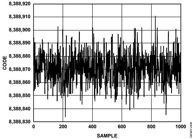
Figure 8. Noise ( V_{REF} = AV_{DD} = 5\text{ V} , Output Data Rate = 2400 Hz, Gain = 1, Chop Disabled, \text{Sinc}^4 Filter)
