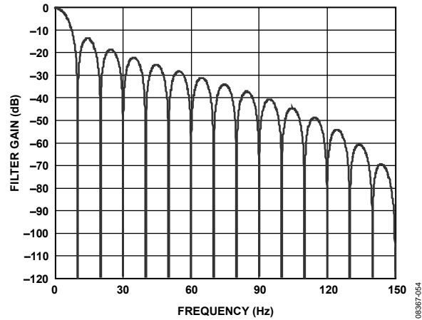
Figure 65. Filter Response for Average + Decimate Filter (Sinc 3 Filter, FS[9:0] = 30, Average by 16)
