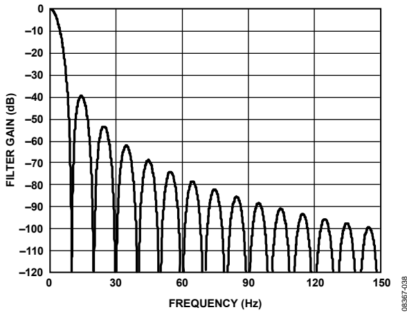
Figure 41. Sinc 3 Filter Response (FS[9:0] = 480)
