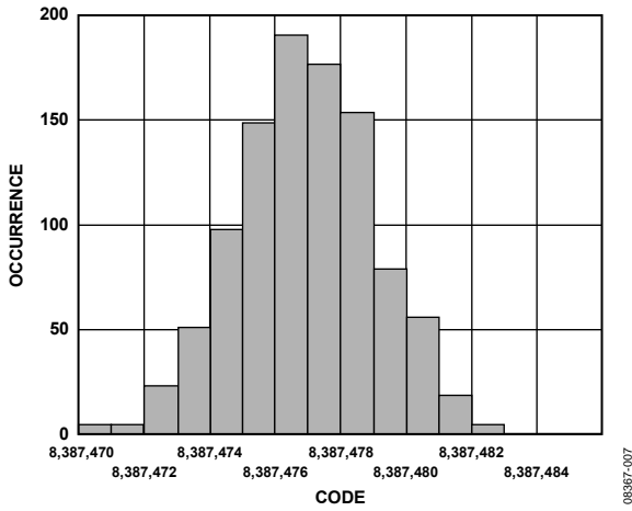
Figure 7. Noise Distribution Histogram ( V_{REF} = AV_{DD} = 5\text{ V} , Output Data Rate = 4.7 Hz, Gain = 128, Chop Disabled, \text{Sinc}^4 Filter)
