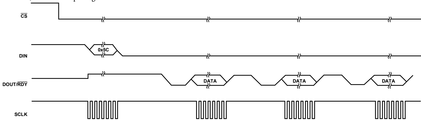
Figure 26. Continuous Read
