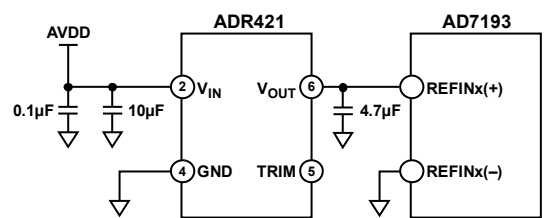
Figure 22. ADR421 to AD7193 Connections
