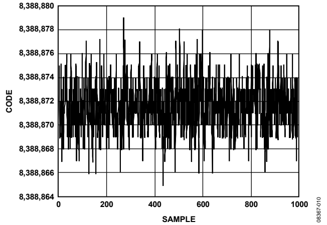
Figure 10. Noise ( V_{REF} = AV_{DD} = 5\text{ V} , Output Data Rate = 42.1 Hz (FS[9:0] = 6, Average by 16), Gain = 1, Chop Disabled, \text{Sinc}^4 Filter)
