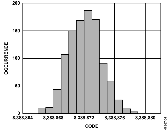
Figure 11. Noise Distribution Histogram ( V_{REF} = AV_{DD} = 5\text{ V} , Output Data Rate = 42.1 Hz (FS[9:0] = 6, Average by 16), Gain = 1, Chop Disabled, \text{Sinc}^4 Filter)
