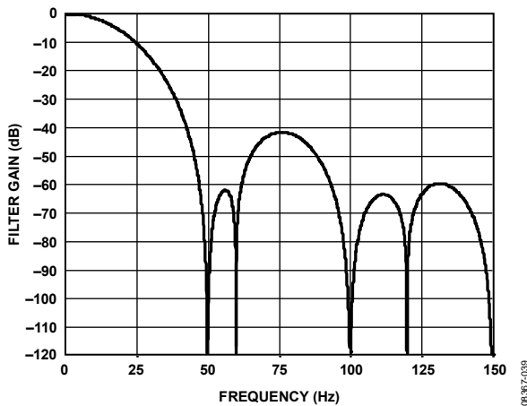
Figure 42. Sinc 3 Filter Response (FS[9:0] = 96, REJ60 = 1)
