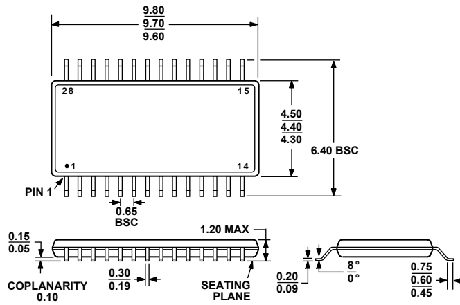
Figure 68. 28-Lead Thin Shrink Small Outline Package [TSSOP] (RU-28)
