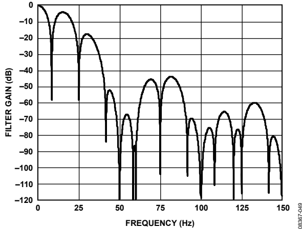
Figure 52. Sinc 3 Filter Response (FS[9:0] = 96, Chop Enabled, REJ60 = 1)
