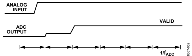
Figure 55. Step Change on Analog Input, Sinc 4 Filter
