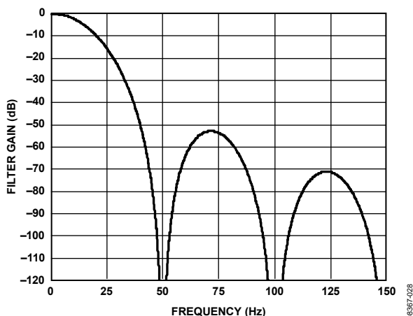
Figure 31. Sinc 4 Filter Response (FS[9:0] = 96)
