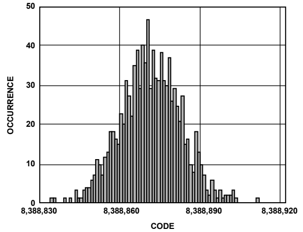
Figure 9. Noise Distribution Histogram ( V_{REF} = AV_{DD} = 5\text{ V} , Output Data Rate = 2400 Hz, Gain = 1, Chop Disabled, \text{Sinc}^4 Filter)
