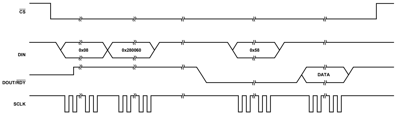
Figure 24. Single Conversion
