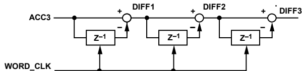
Figure 28. Differentiator
