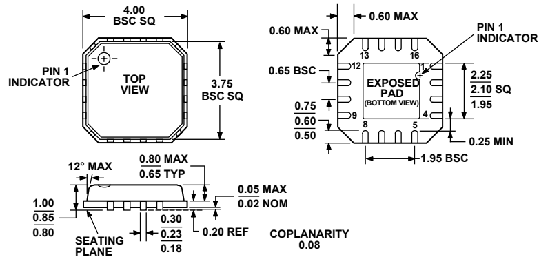
COMPLIANT TO JEDEC STANDARDS MO-220-VGGC Figure 37. 16-Lead Lead Frame Chip Scale Package [LFCSF_VQ] 4 mm × 4 mm Body, Very Thin Quad (CP-16-4) Dimensions shown in millimeters
