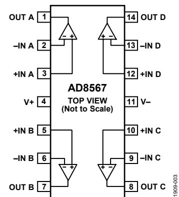
Figure 3. 14-Lead TSSOP Pin Configuration
