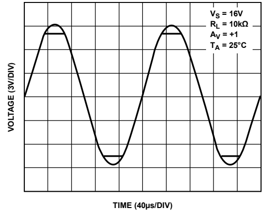
Figure 21. No Phase Reversal
