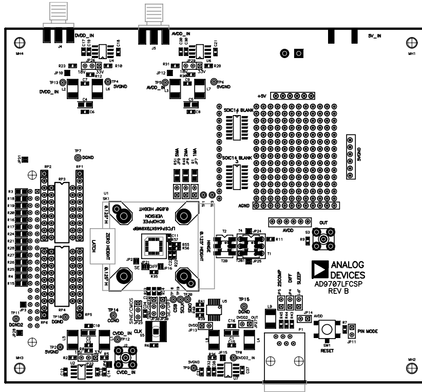
Figure 97. Assembly—Primary Side
