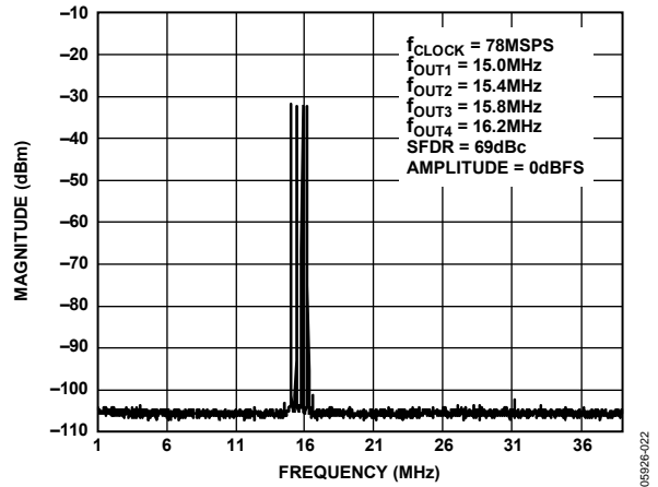
Figure 26. Four-Tone SFDR
