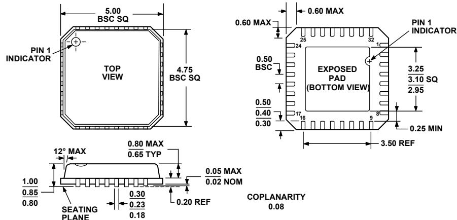
Figure 103. 32-Lead Lead Frame Chip Scale Package [LFCSP_VQ] 5 mm × 5 mm, Very Thin Quad (CP-32-2) Dimensions shown in millimeters
