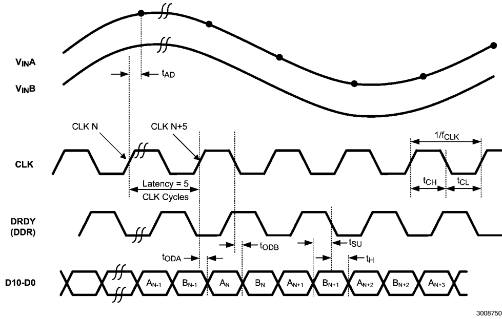
FIGURE 1. LVDS Output Timing
