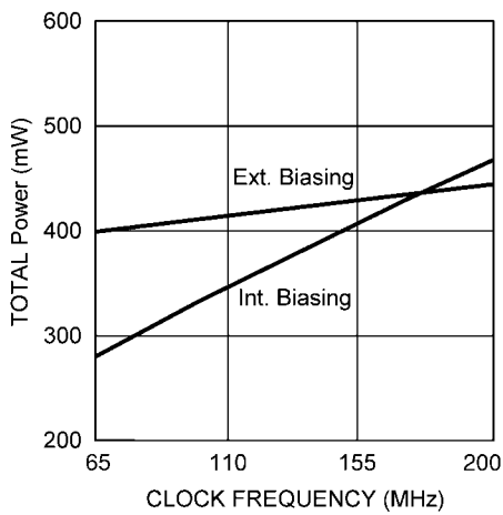
Total Power vs. Clock Frequency, f_{IN} = 10 MHz
