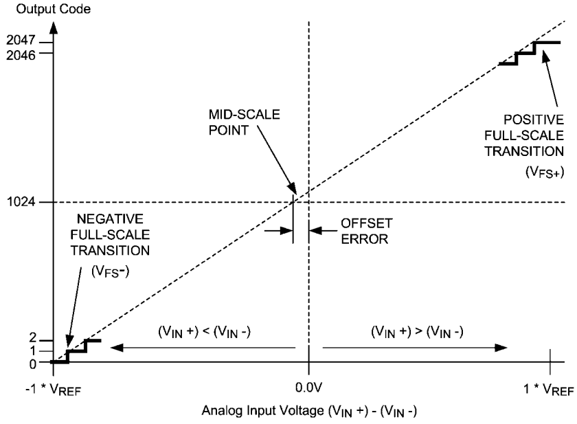
FIGURE 3. Transfer Characteristic
