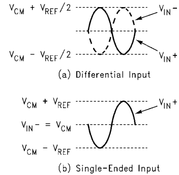
FIGURE 2. Expected Input Signal Range
