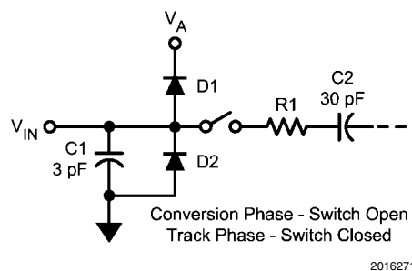
FIGURE 7. Equivalent Input Circuit
