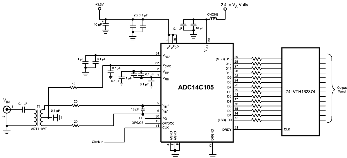
FIGURE 7. Application Circuit
