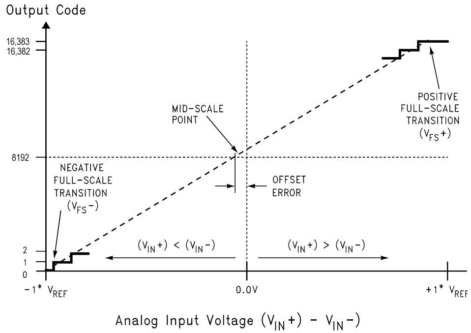
FIGURE 1. Transfer Characteristic
