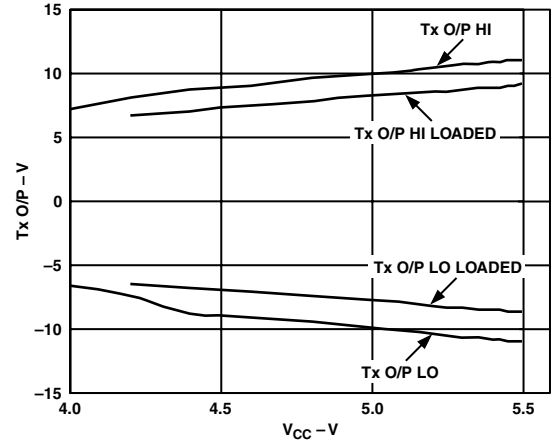
TPC 4. Transmitter Output Voltage vs. V_{CC}
