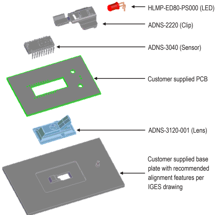
Figure 5. Exploded view
