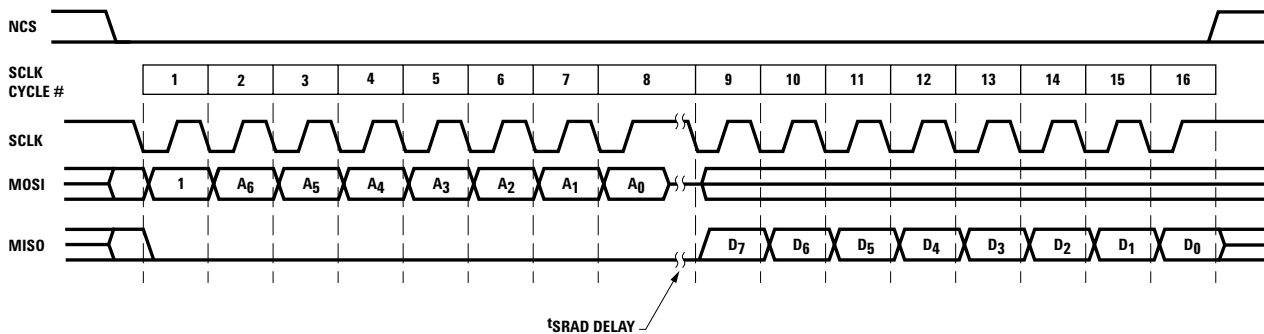
Figure 16. Read operation.
