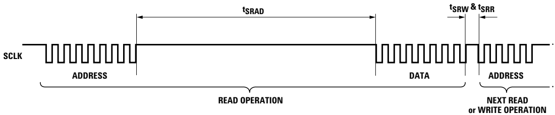
Figure 20. Timing between read and either write or subsequent read
