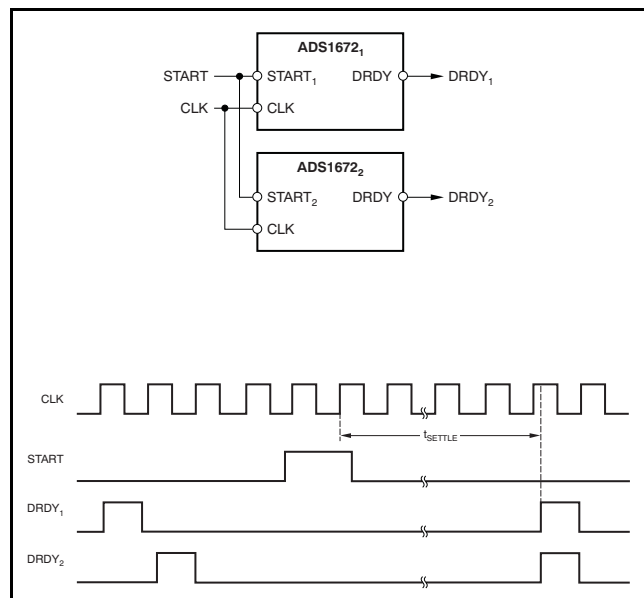
Figure 38. Synchronizing Multiple Converters
