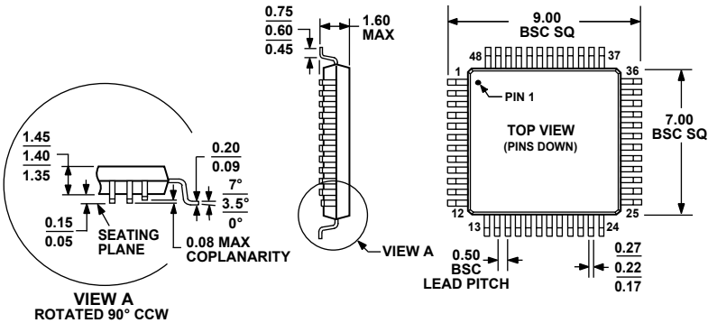
Figure 46. 48-Lead Low Profile Quad Flat Package [LQFP] (ST-48)
