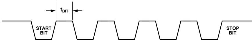
Figure 41. LIN Sync Byte Field
