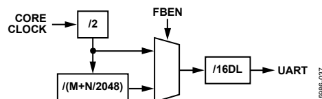
Figure 37. Fractional Divider Baud Rate Generation
