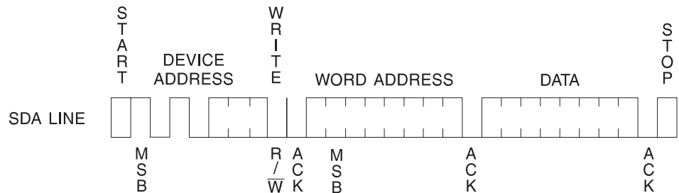
Figure 11. Byte Write
