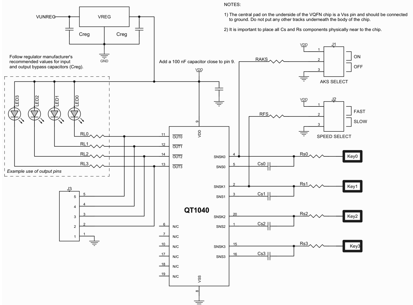
Figure 1-1. Typical Circuit
