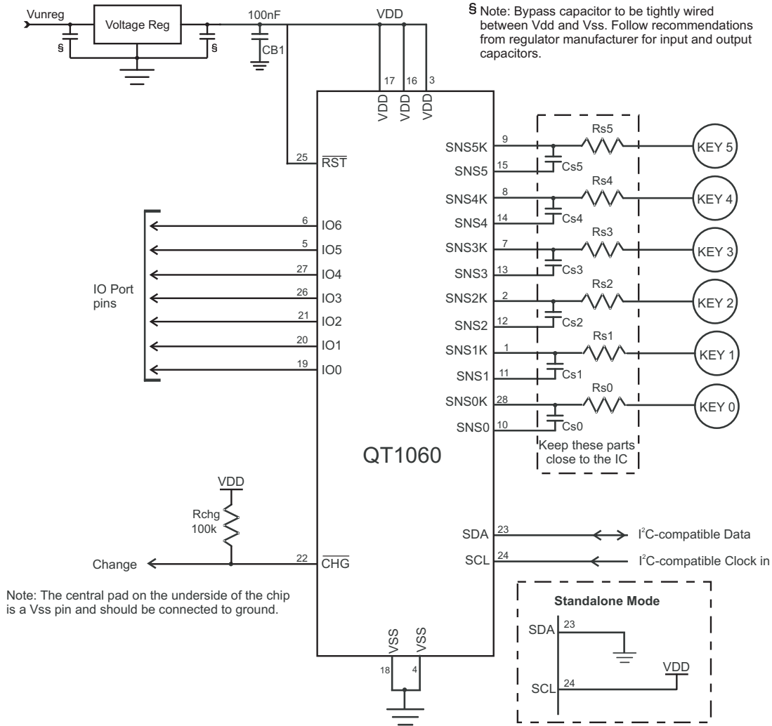
Figure 1-1. Typical Circuit
