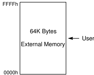
Figure 6-2. AT80C51SND1C Memory Architecture
