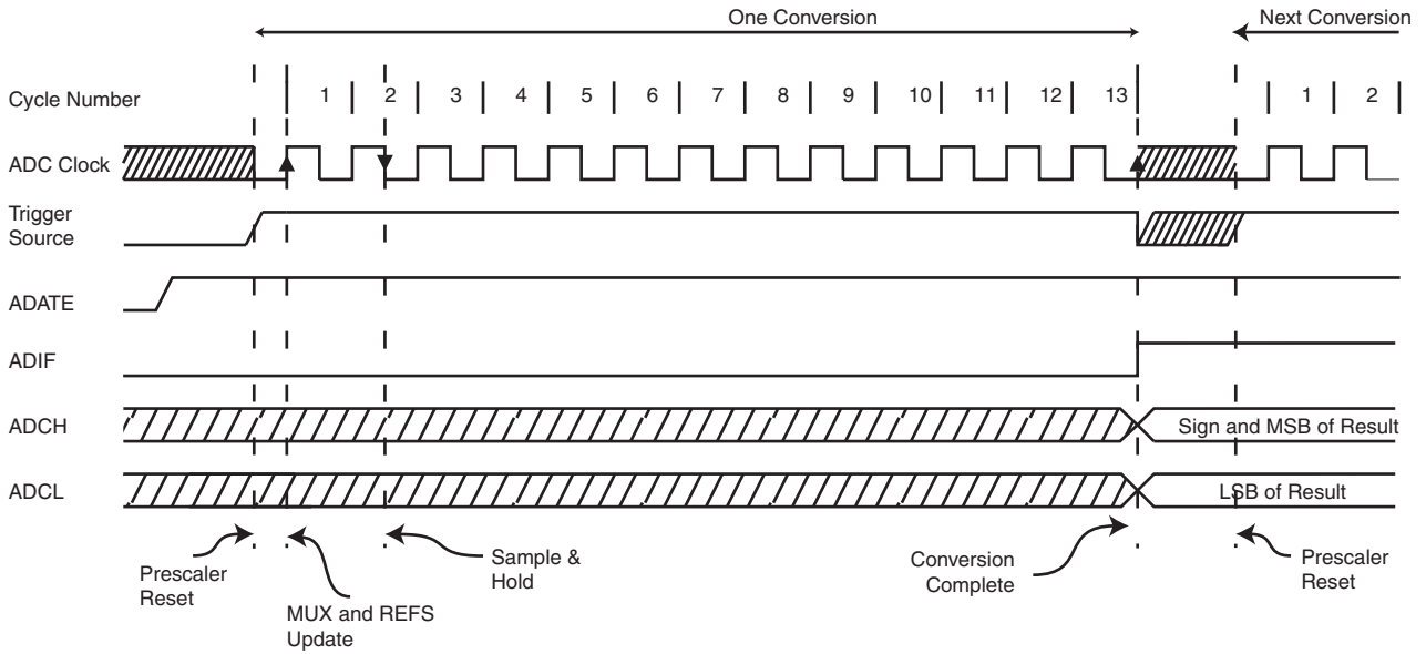
Figure 4-87. ADC Timing Diagram, Auto Triggerred Conversion
