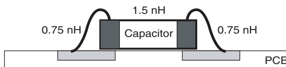
Figure 4-114. Capacitor Description
