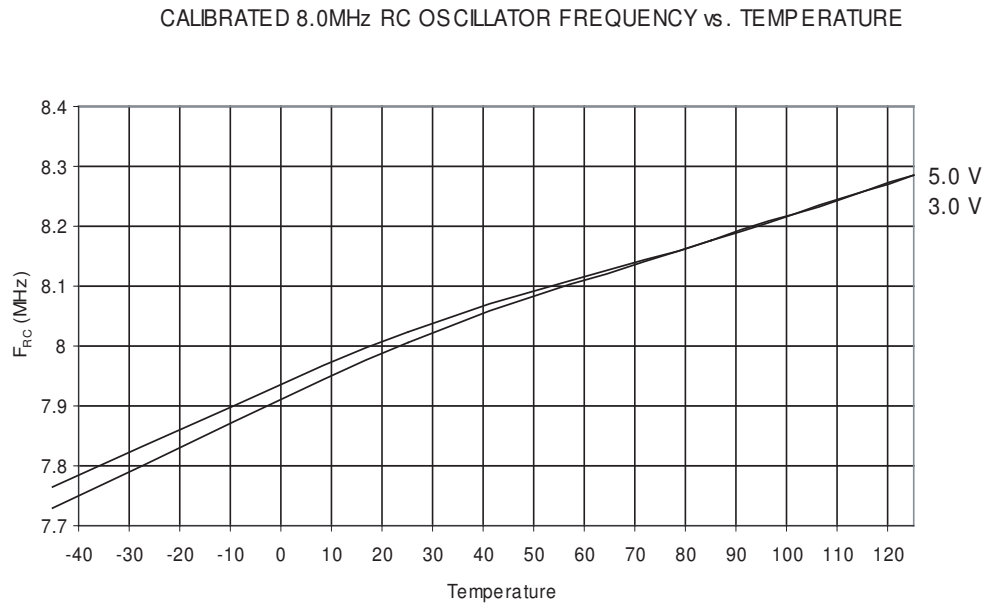
Figure 23-34. Calibrated 8 MHz RC oscillator Frequency vs. Temperature
