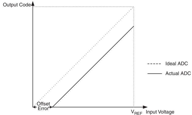
Figure 19-9. Offset Error
