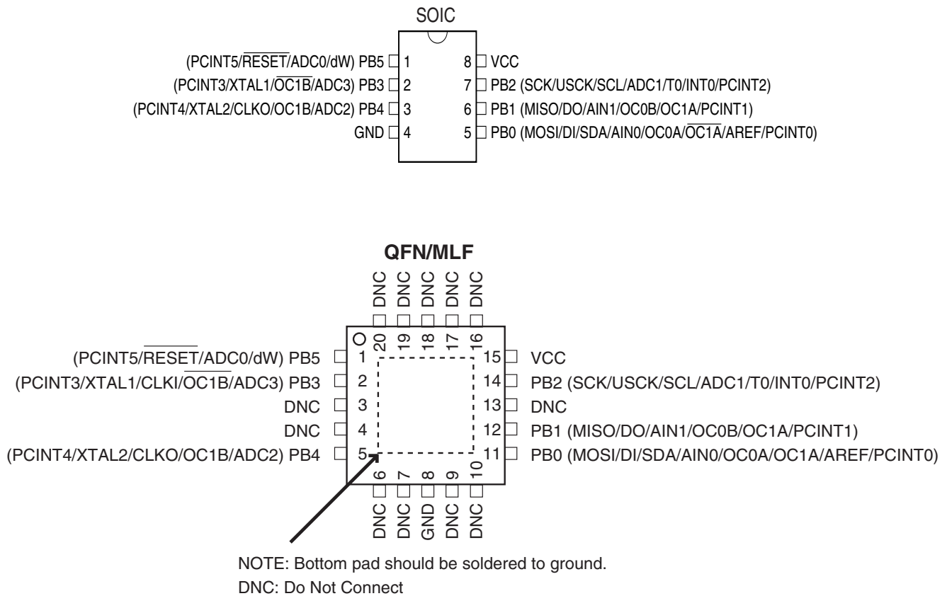
Figure 1-1. Pinout ATtiny25/45/85
