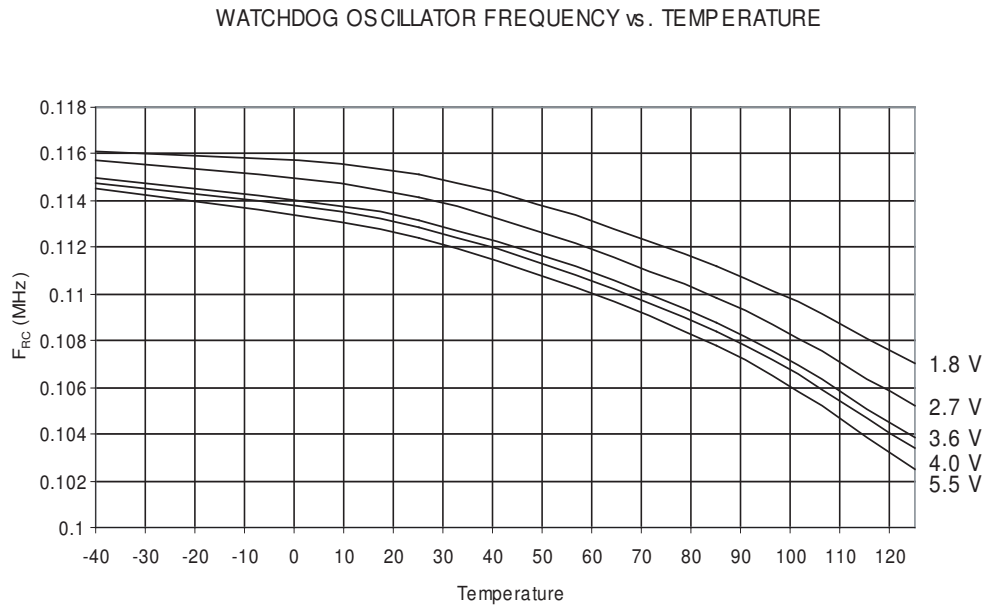
Figure 24-35. Watchdog Oscillator Frequency vs. Temperature
