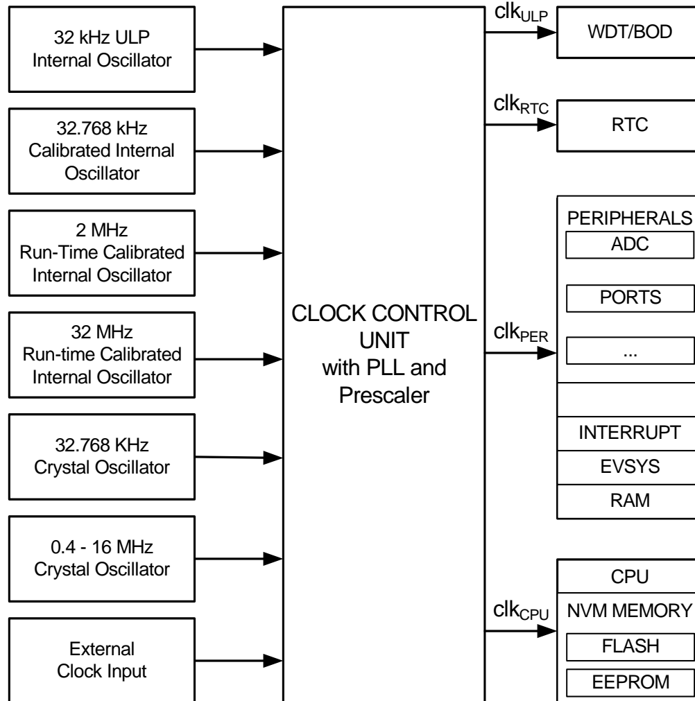
Figure 9-1. Clock system overview
