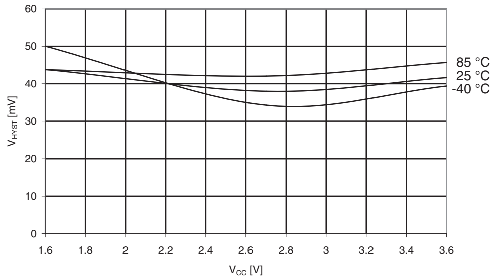
Figure 32-35. Analog Comparator Hysteresis vs. V_{CC} High-speed, Large hysteresis.
