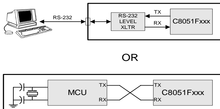
Figure 22.3. UART Interconnect Diagram
