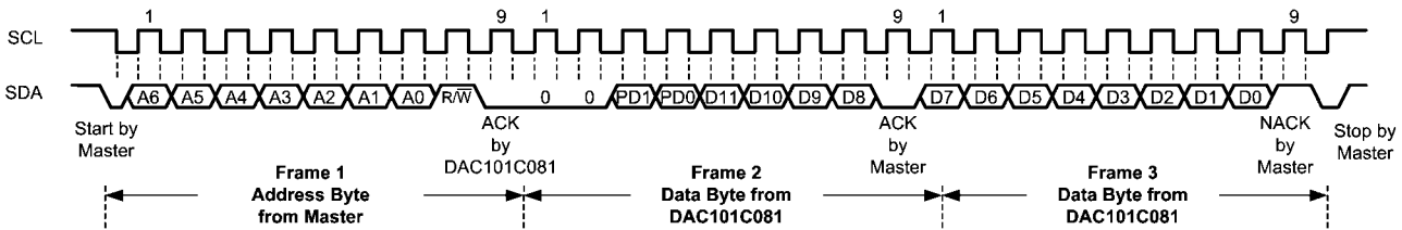
FIGURE 7. Typical Read from the DAC Register
