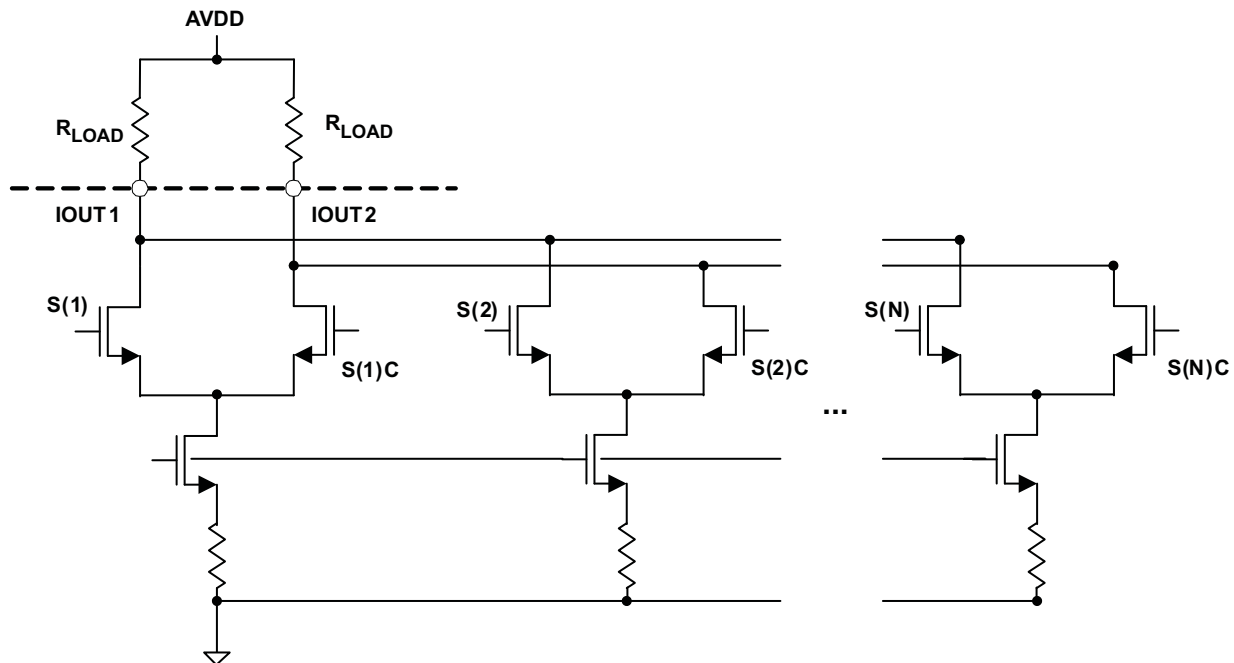
Figure 41. Equivalent Analog Current Output
