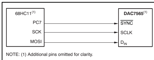
Figure 103. DAC7565 to 68HC11 Interface
