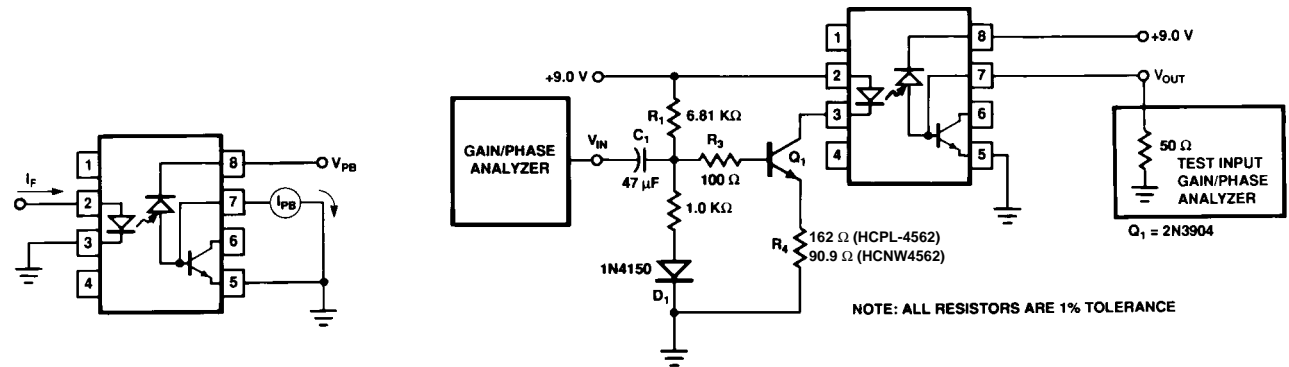
Figure 2. Base photo current test circuit.
