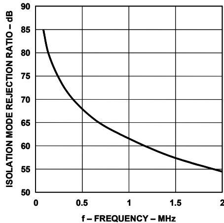
Figure 6. Isolation mode rejection ratio vs. frequency
