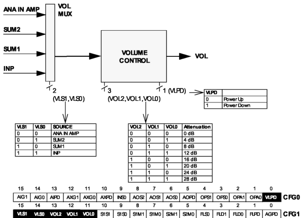
Figure 9: Volume Control
