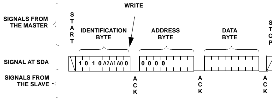
FIGURE 13. ACKNOWLEDGE RESPONSE FROM RECEIVER
