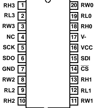
ISL22444 (20 LEAD TSSOP) TOP VIEW
