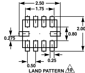
LAND PATTERN 10
