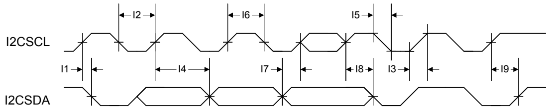
Figure 20-2. I 2 C Timing
