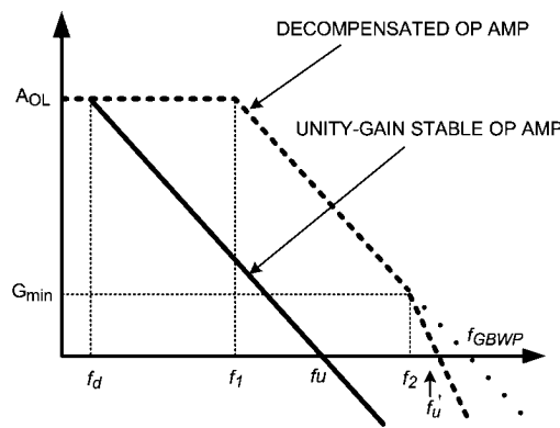
Increased Bandwidth for Same Supply Current at A_V > 10
