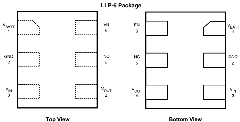
FIGURE 5: Connection Diagram 6-Pin Chip On Lead LLP package, 0.5mm pitch See NS Package Number LCA06B
