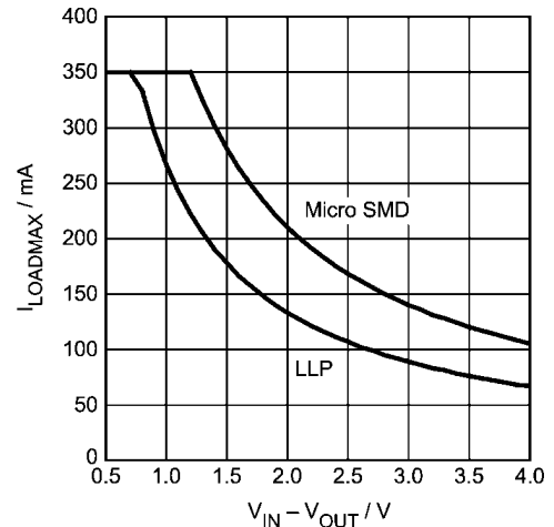
FIGURE 7: Maximum Load Current vs V_{IN} - V_{OUT} , T_A = 85^\circ\text{C} , V_{OUT} = 1.5\text{V} , \theta_{JA(\text{MICROSMD})} = 95^\circ\text{C/W} , \theta_{JA(\text{LLP})} = 150^\circ\text{C/W} , 20208525
