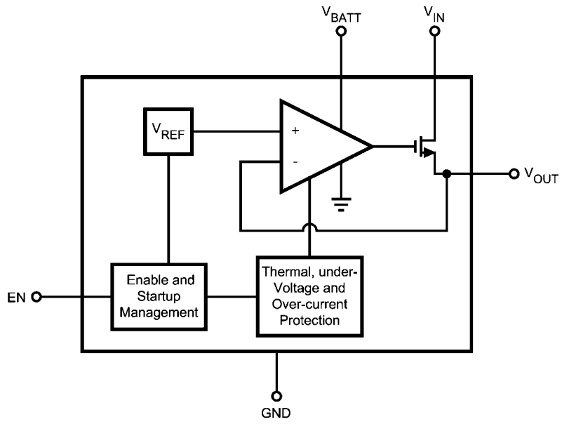
FIGURE 6: Block Diagram
