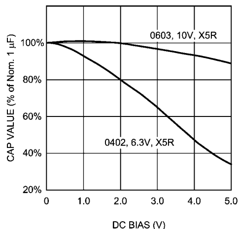
FIGURE 8: Graph Showing A Typical Variation In Capacitance vs DC Bias
