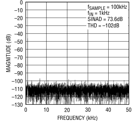
LTC1854 Nonaveraged 4096-Point FFT Plot
