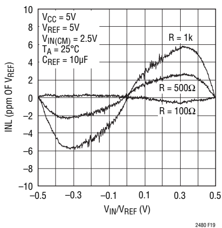
Figure 19. INL vs Differential Input Voltage and Reference Source Resistance for C_{REF} > 1\mu F
